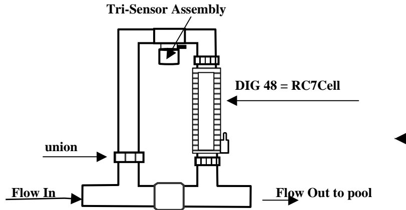
Flow Bypass Manifold Assembly
