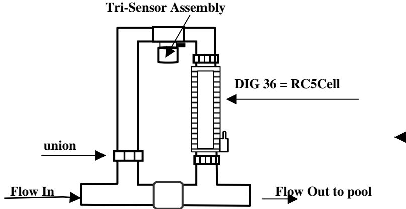
Flow Bypass Manifold Assembly
